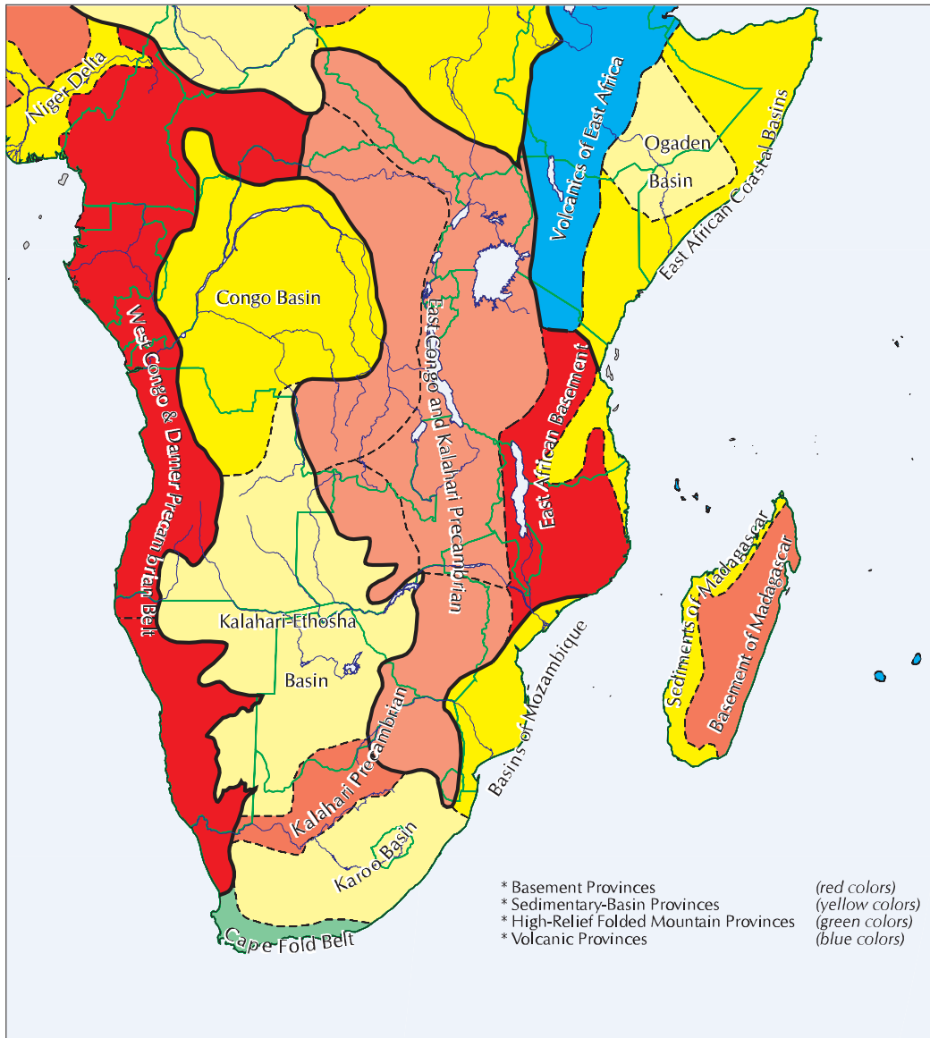
Proposed Groundwater Provinces
